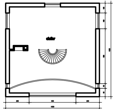
KIBİ PLANI
