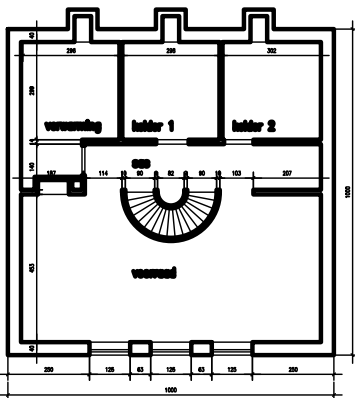
KIBİ PLANI
